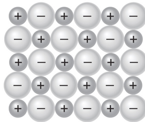
Ionic lattice (a)
