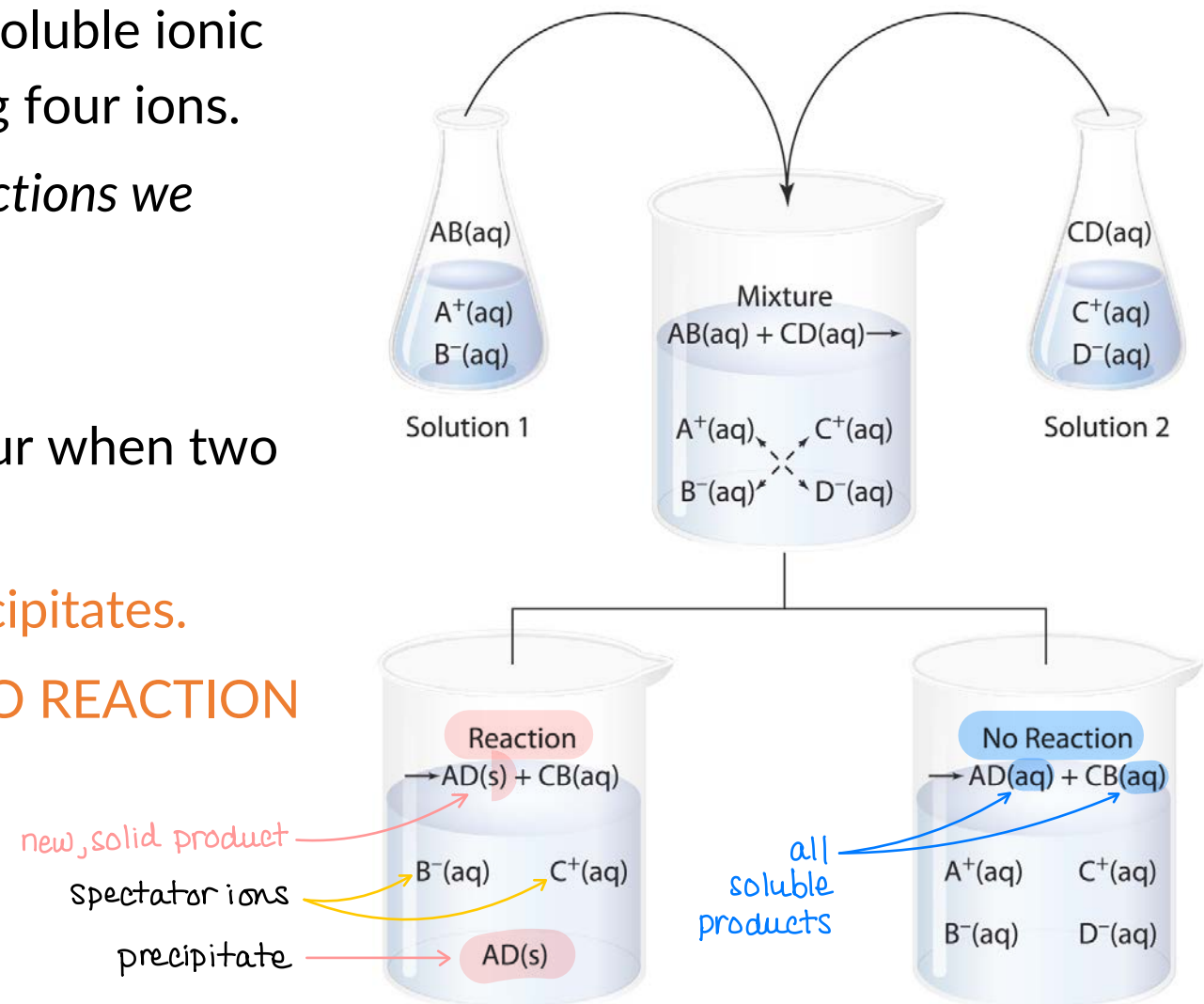
FIGURE 4.19 Two Solutions of Ionic Compounds
